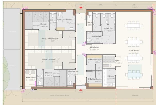
Proposed Ground Floor Plan 1:100
