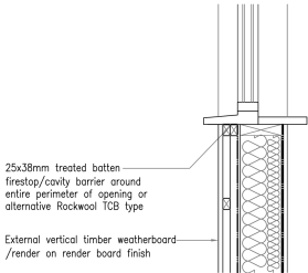
Window Section Detail 1
