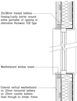
Window Section Detail 2 (weatherboard)
