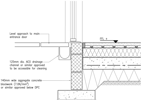
Typical Flush Threshold Detail
