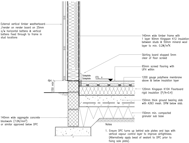
Typical Foundation / Ground Floor Detail
