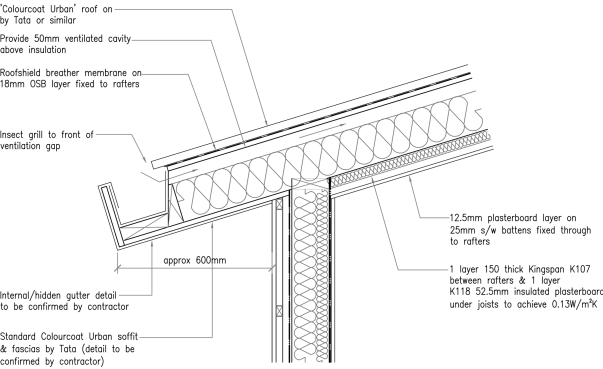
Typical Roof Detail
