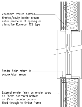
Window Section Detail 2 (render)
